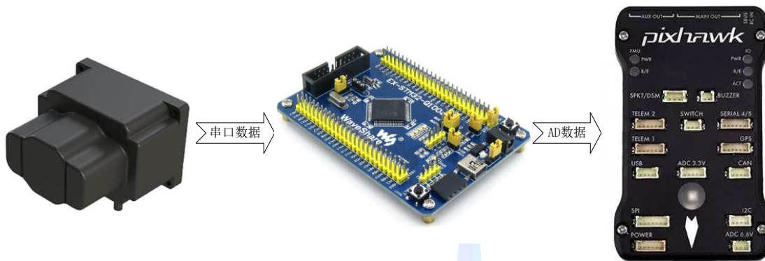
Pic. 4 connect TF SERIES to PixHawk
